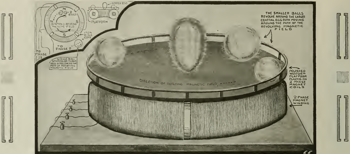
Fig. 2. Illustrating the Polyphase Coil and Rotating Magnetic Field Which Caused Copper Eggs to Spin. Fig. 3. Insert: Detail of Coil Apparatus Showing Coil Connections to Different Copper Phases.
