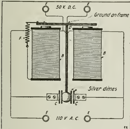
Simple Rectifier Constructed From Polarized Ringer.
