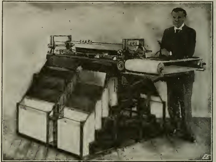
Another View of the Electric Tobacco Leaf Sorting Machine. Two Leaves Can Be Seen Sliding Down Toward the Open Compartments. The Inventor Is Seen Operating the Machine.
