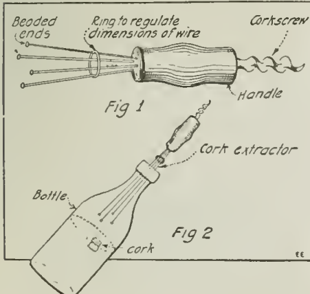
Clever Combination Cork Screw and Cork Extractor.
