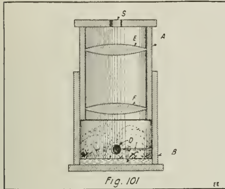
The Crookes "Spintharoscope," Which Demonstrates in a Popular Way the Wonders of Radium. These Can Be Purchased On the Market.
