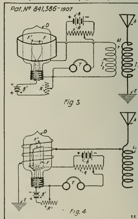
The First "Three Electrode" Audion Had a Piece of Tin-foil Wrapt Around the Outside of the Bulb—a Principle Frequently "Rediscovered," as Was the de Forest Electro-magnetic or Coil Electrode, Fig. 4.
