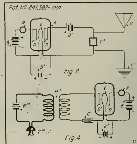
Here We Find the "Third Electrode" Placed Inside the Bulb, Where It Logically Belonged, as Dr. de Forest Points Out. Fig. 4 Shows the First Use of the "Stopping" Condenser.
